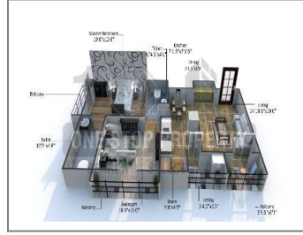
Floor Plan
